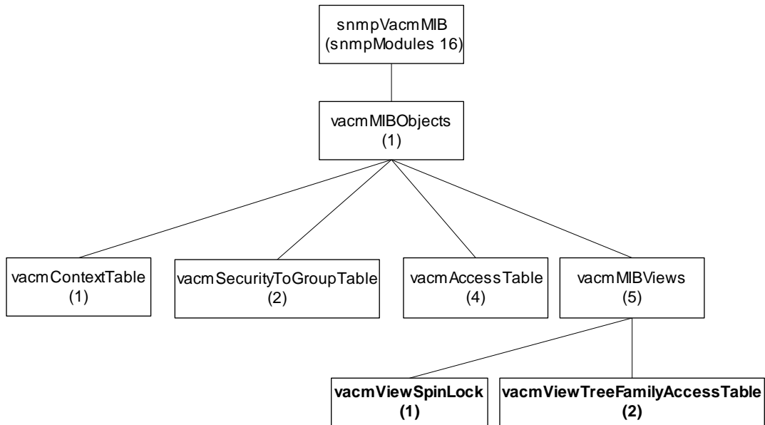
Figure 7.17 VACM MIB
