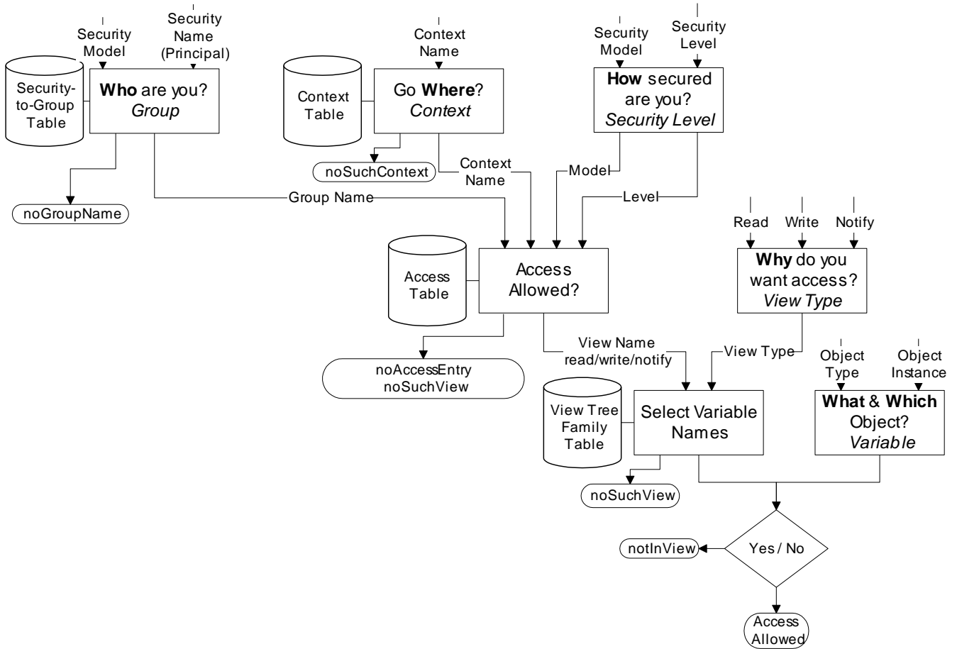
Figure 7.16 VACM Process
