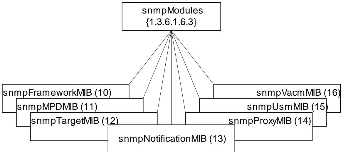
Figure 7.7 SNMPv3 MIB
