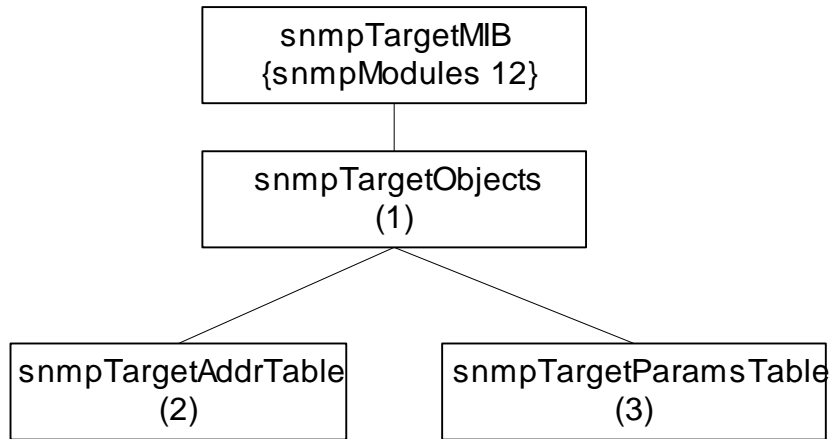
Figure 7.8 Target Address and Target Parameter Tables
